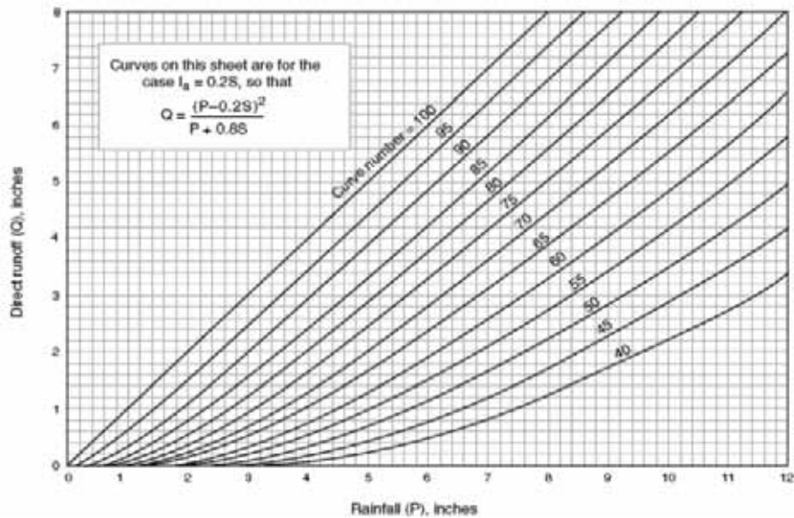
Figure 2-1 Solution of runoff equation.
