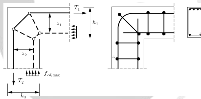
(a)기둥과보의깊이가동일한경우
