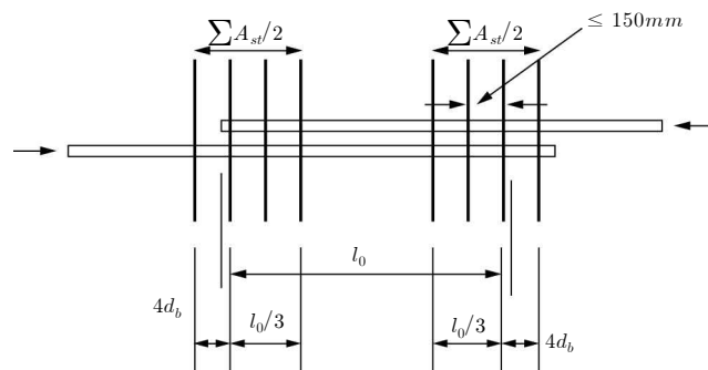
(b) 압축철근
